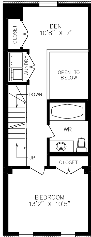
THIRD FLOOR 507 SQUARE FEET
