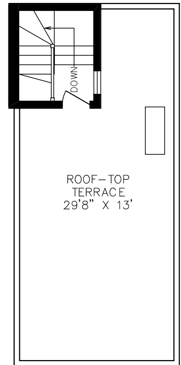
FOURTH FLOOR 65 SQUARE FEET
